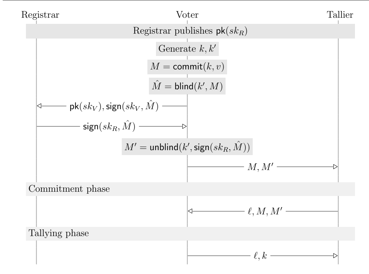
Figure 3.1 FOO electronic voting protocol
